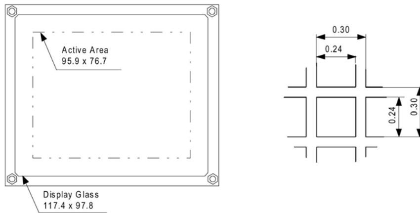
Fig 5. Viewing Area Characteristics in mm.
