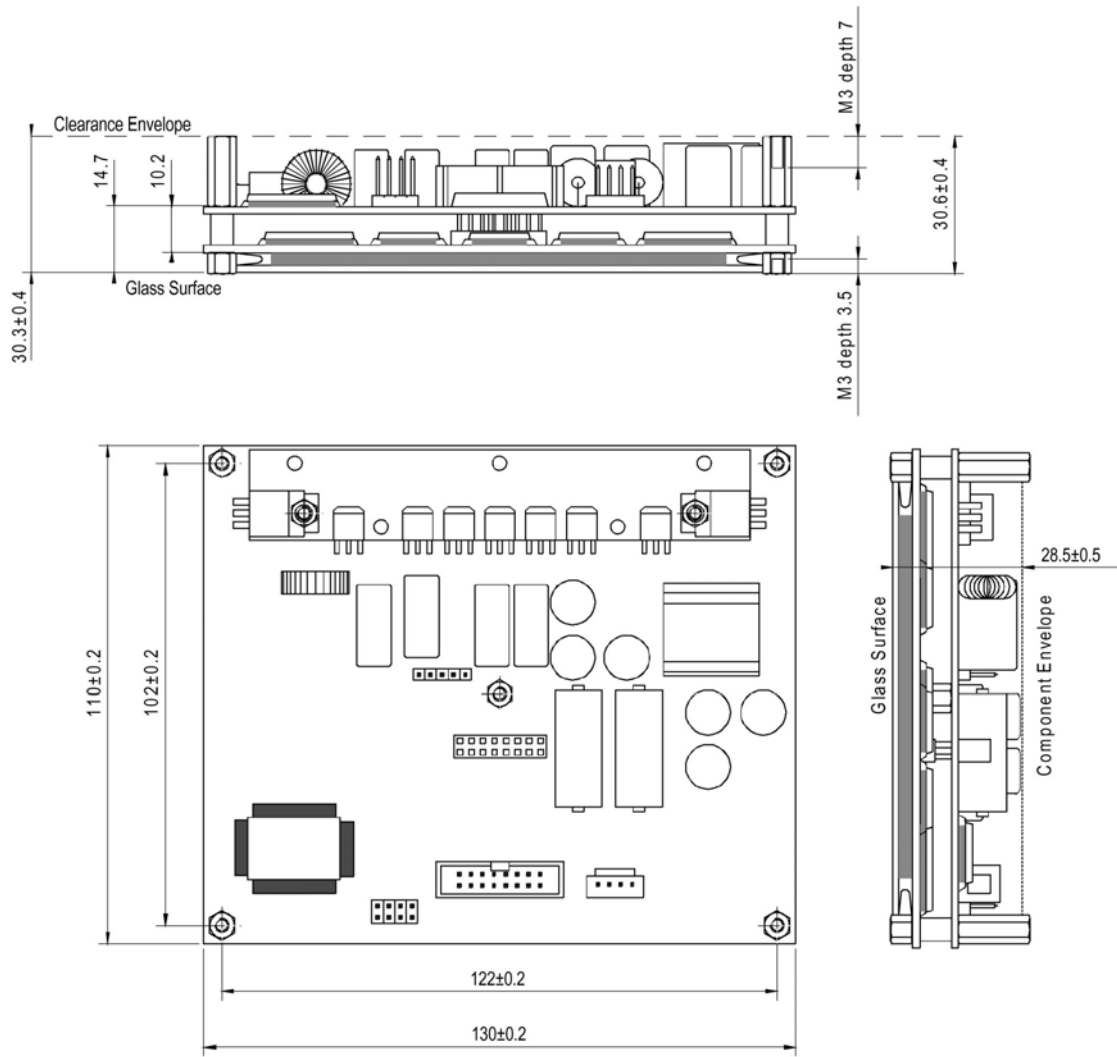
Fig 6. Mechanical dimensions in mm.
