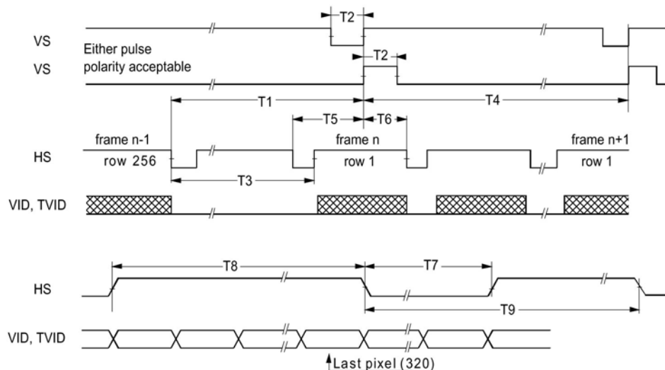
Figure 3. Timing Characteristics
