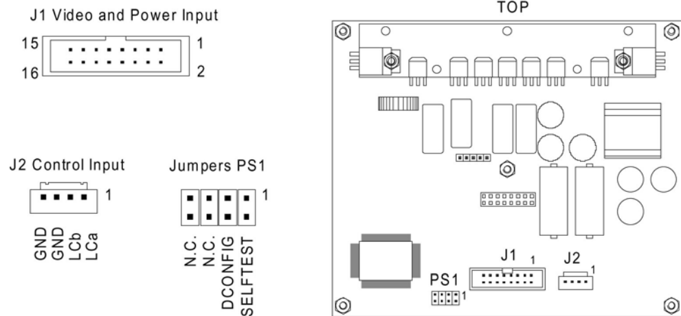
Fig 2. Input Connectors and Programmable Jumpers.
